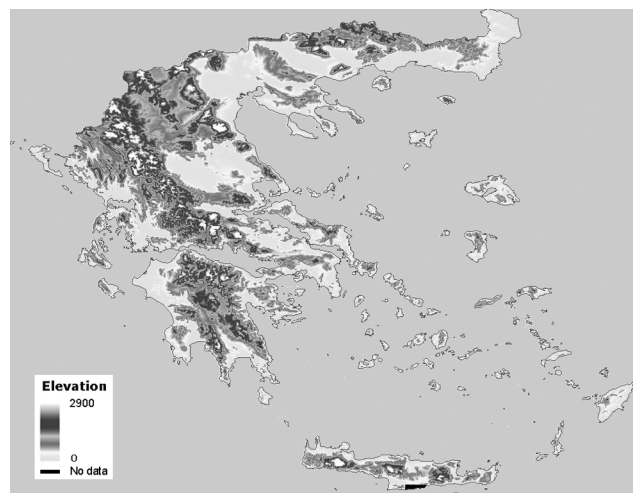
Figure 2. A DEM for Greece that was generated using the GDEM tiles.
